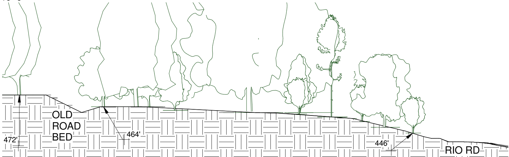
2 ROCKBROOK SECTION 2 1" = 40'-0"
